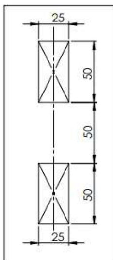
PANEL CUTOUT
